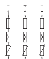
VG-C DCPH1000-4S
