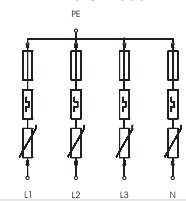
V20-C 4-550
