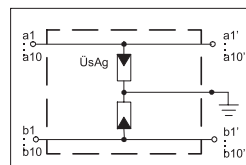
LSA-B-MAG
